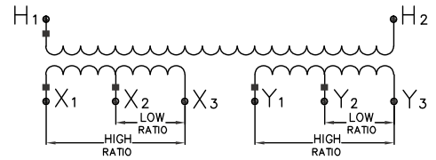
Dual-Tapped Secondary (Six secondary terminals)
